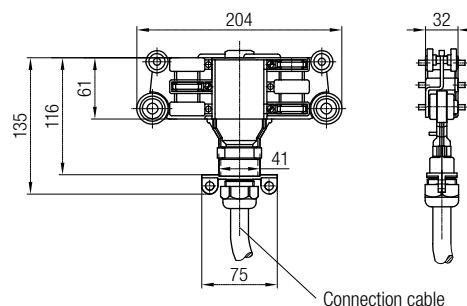
Connection cable
